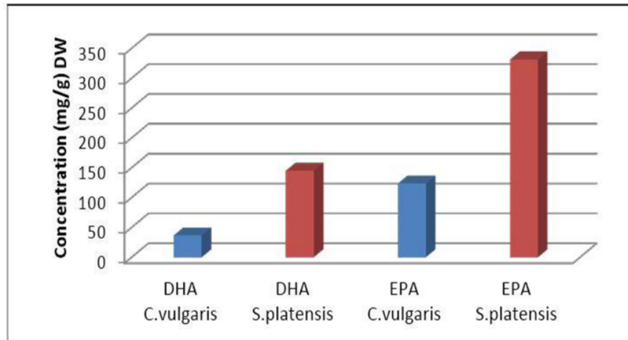
Figure 3: The concentration of DHA and EPA in C.vulgaris and S.platensis
